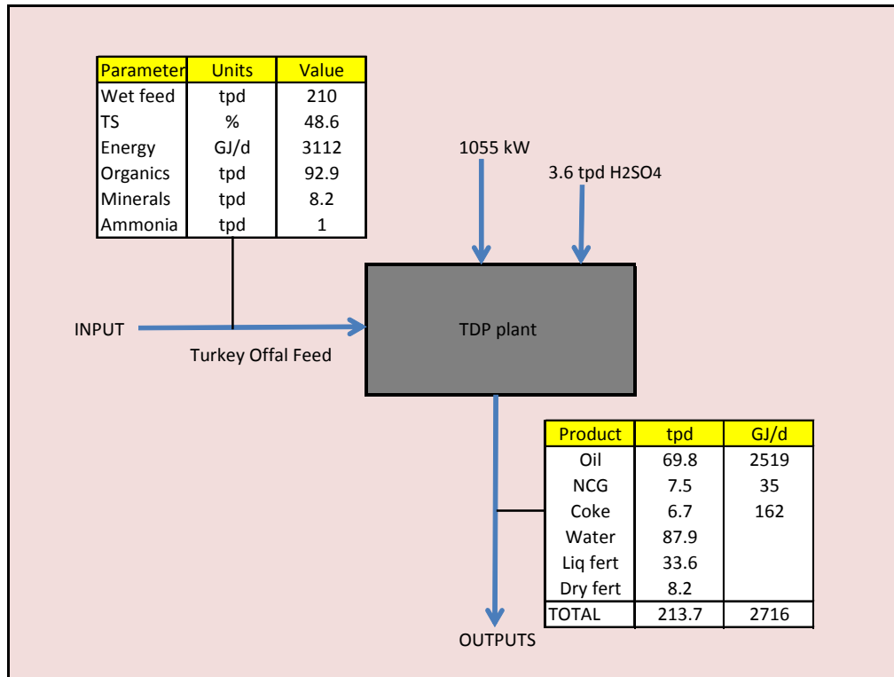
Figure 4.11: Design Inputs and Outputs for the CWT TDP Plant
