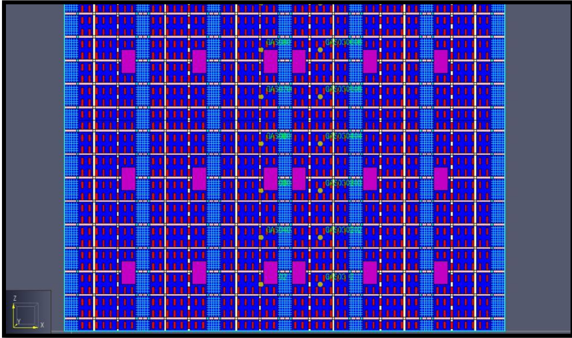
Figure 13. Close up plan view of 36 m deck rear section showing thermocouples and individual sheep. The underside of the sheep is shown in red to indicate heat generation ( 0.427 \text{ kW/m}^2 ) and water vapour evolution ( 0.3542 \text{ g/(m}^2\cdot\text{s)} ) from this surface.
