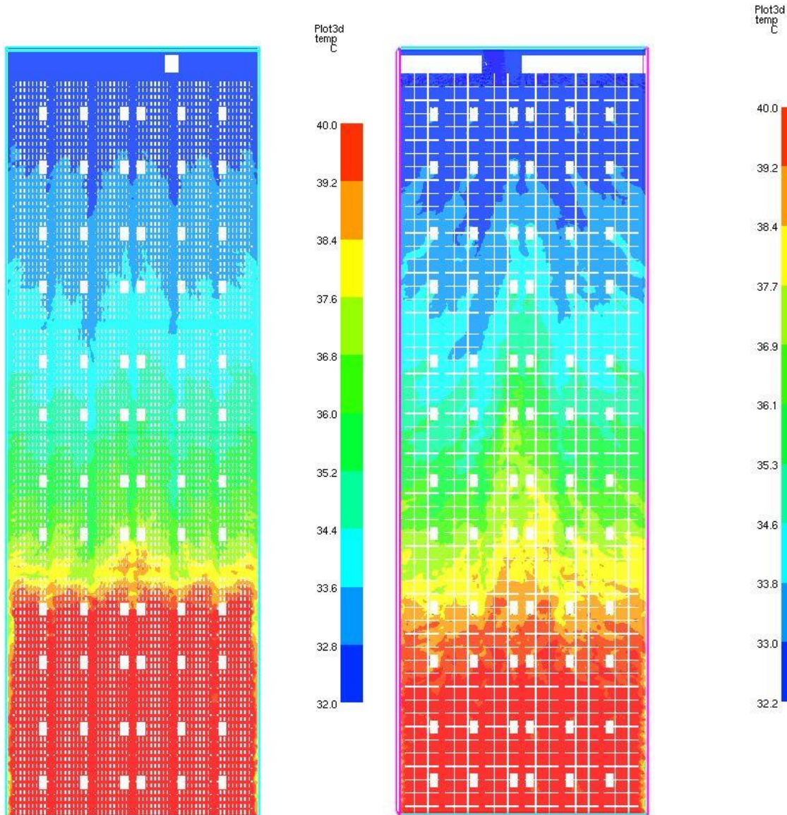
Figure 25. Effect of mechanical ventilation at a PAT of 30 m/hr (right image). The left image has no mechanical ventilation. Temperature scaled up to 40°C. 36 m deck, 20 knot (10.28 m/s) headwind.
