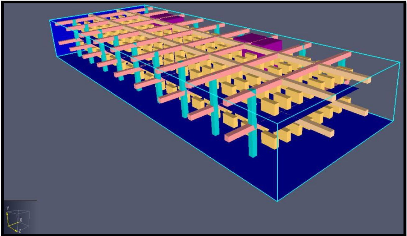
Figure 10. Unit pen (18 m x 6 m x 2.4 m) showing sheep (gold), ventilation risers (purple), vertical structural beams (light blue), cross beams (pink), lengthwise beams (light brown), lower and intermediate decks (dark blue).
