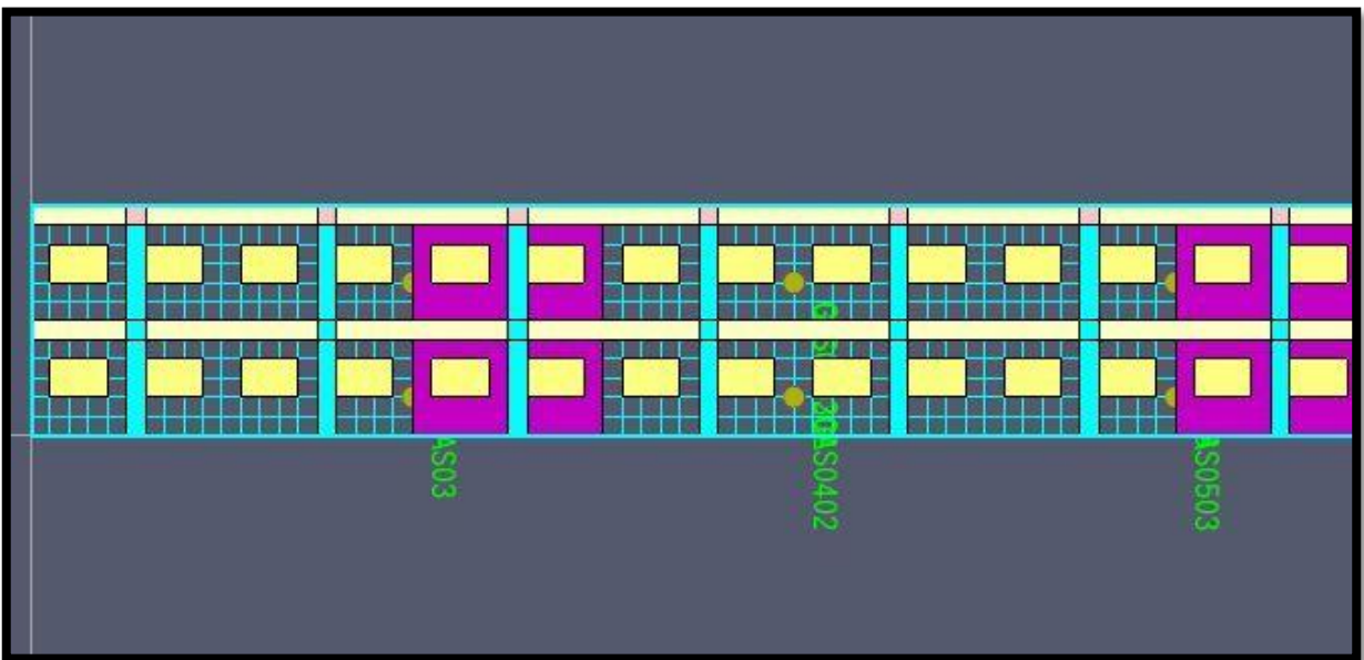
Figure 16. Side view of double deck showing sheep, ventilation risers, structural beams and thermocouple locations.
