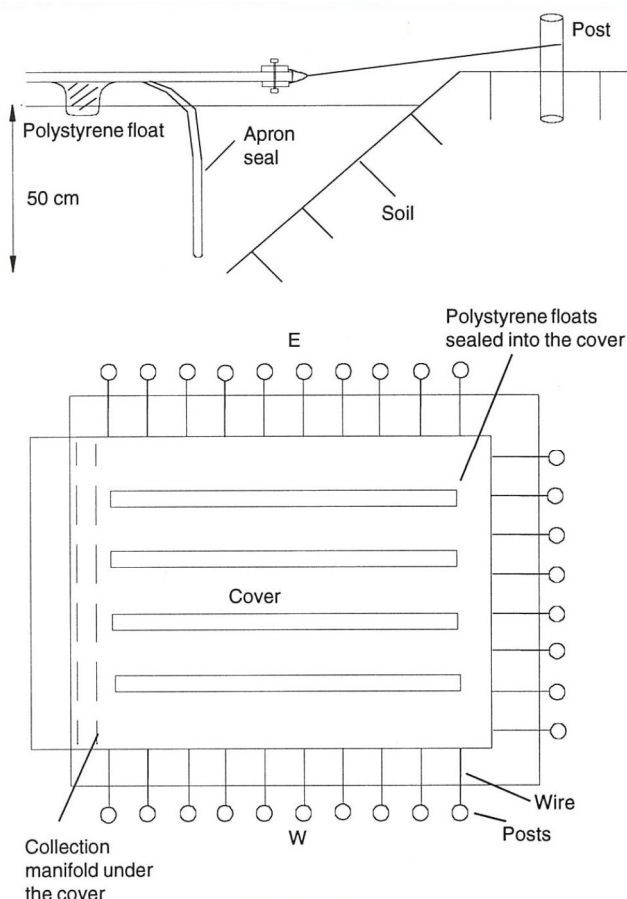
Figure 1 Floating cover installation gas seal
