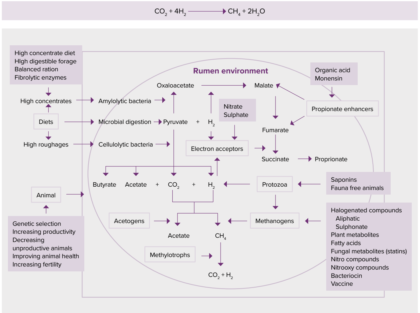
Figure 5: Possible mitigation strategies to reduce CH 4 emissions in rumen fermentation
