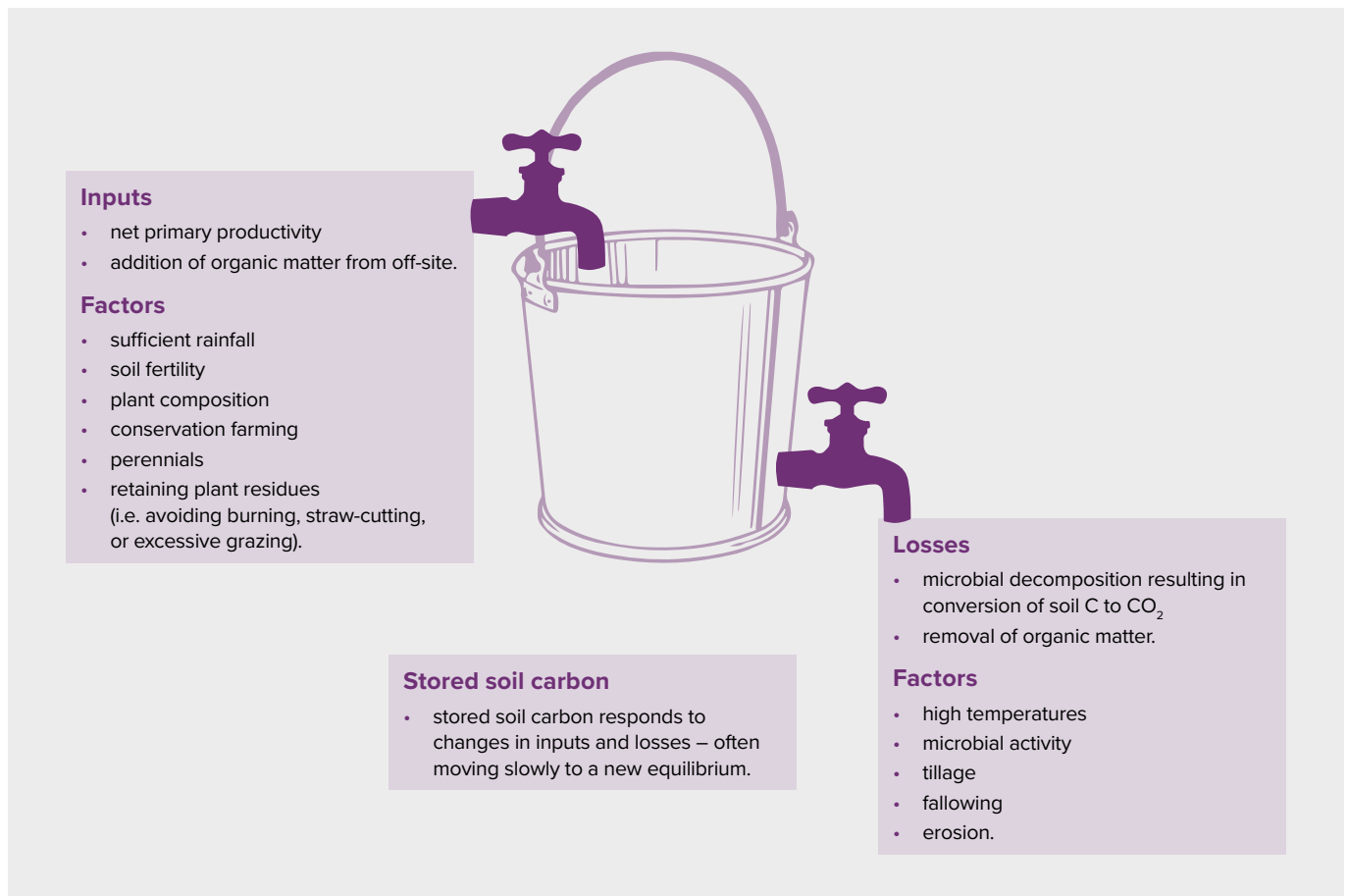
Figure 8: The storage of soil carbon is determined by potential storage, inputs into the soil and losses from the soil
